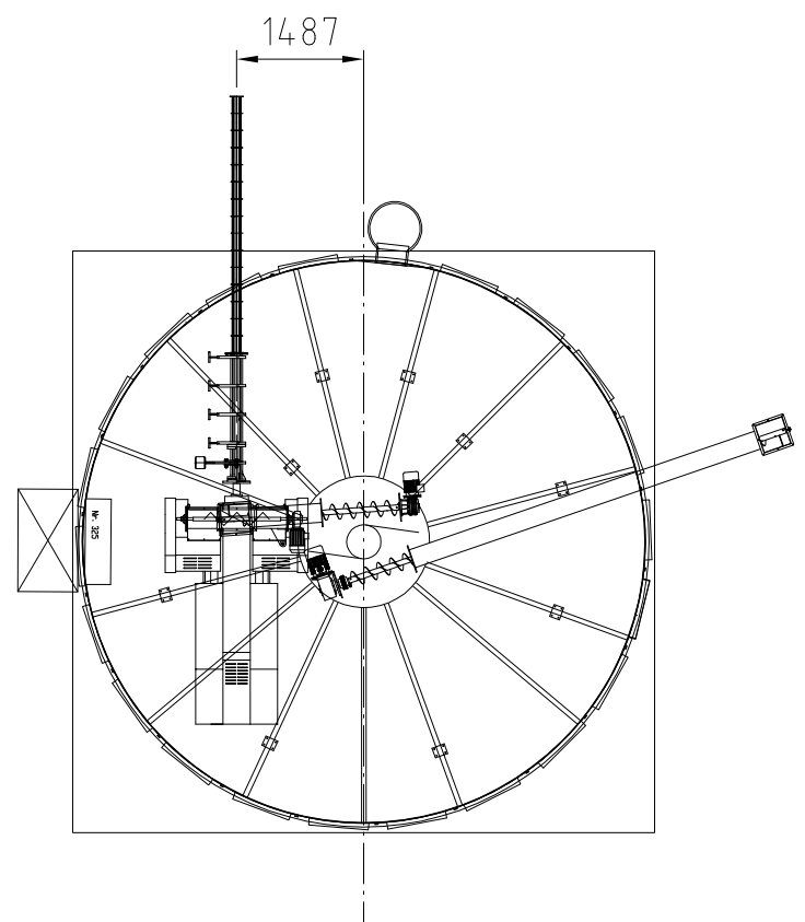
BP6000, dosing screw, emergency screw and placement of silo legs
