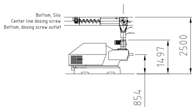
BP6000 and dosing screw
